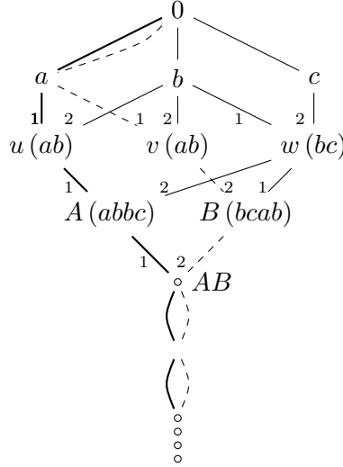
FIGURE 2. A nondeterministic bounded width very untimed system
