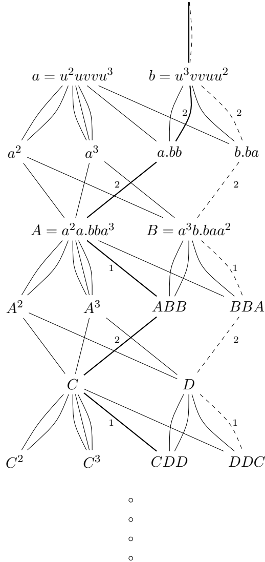
FIGURE 1. Part of a diagram whose system satisfies the old definition of SNE but not the new one
