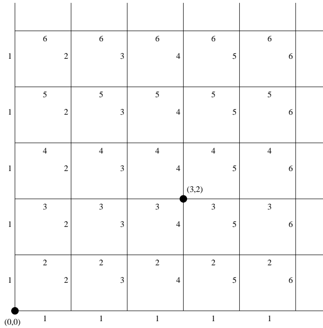
FIGURE 1. The first part of the Euler graph. Numbers along edges indicate multiple edges.
