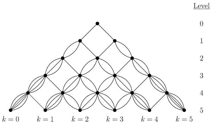
Fig. 6. The reverse Euler graph.
